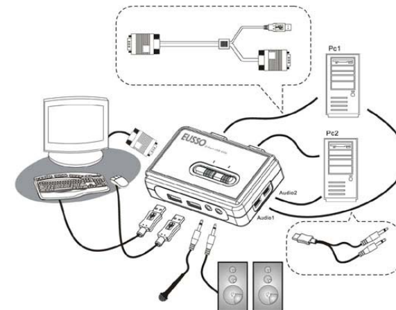
UKS8202-U2/ UKS8202-U2B Configuration Diagram
